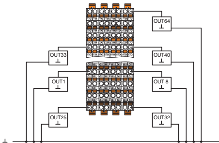
Connection in 1-conductor technology
